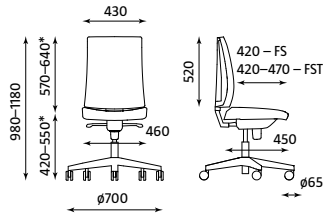
NAVIGO UPH FS RTS TS25 (ST44) ESH Weight | Gewicht: 14.65 kg (14.90 kg) NAVIGO MESH/MESH PLUS Weight | Gewicht: 14.15 kg (14.40 kg)
